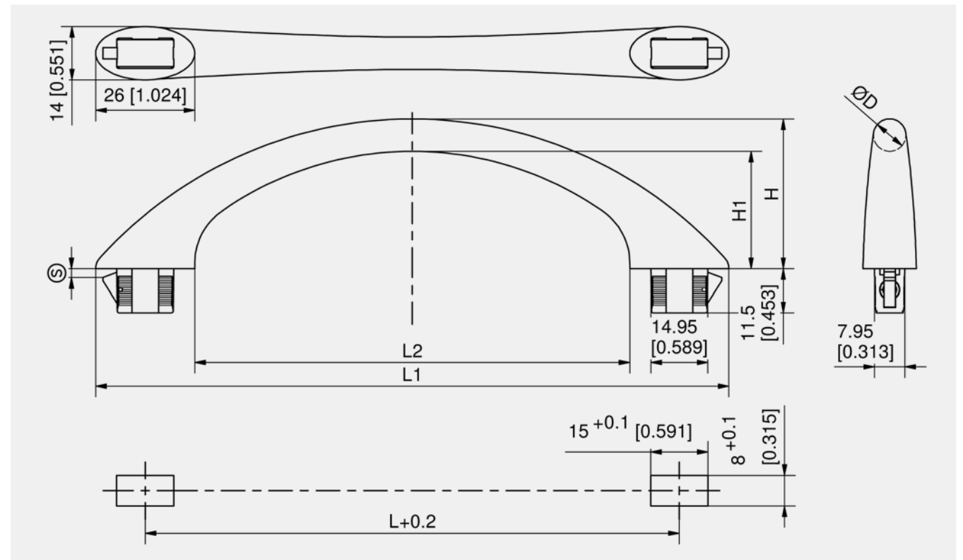
Bridge handle
