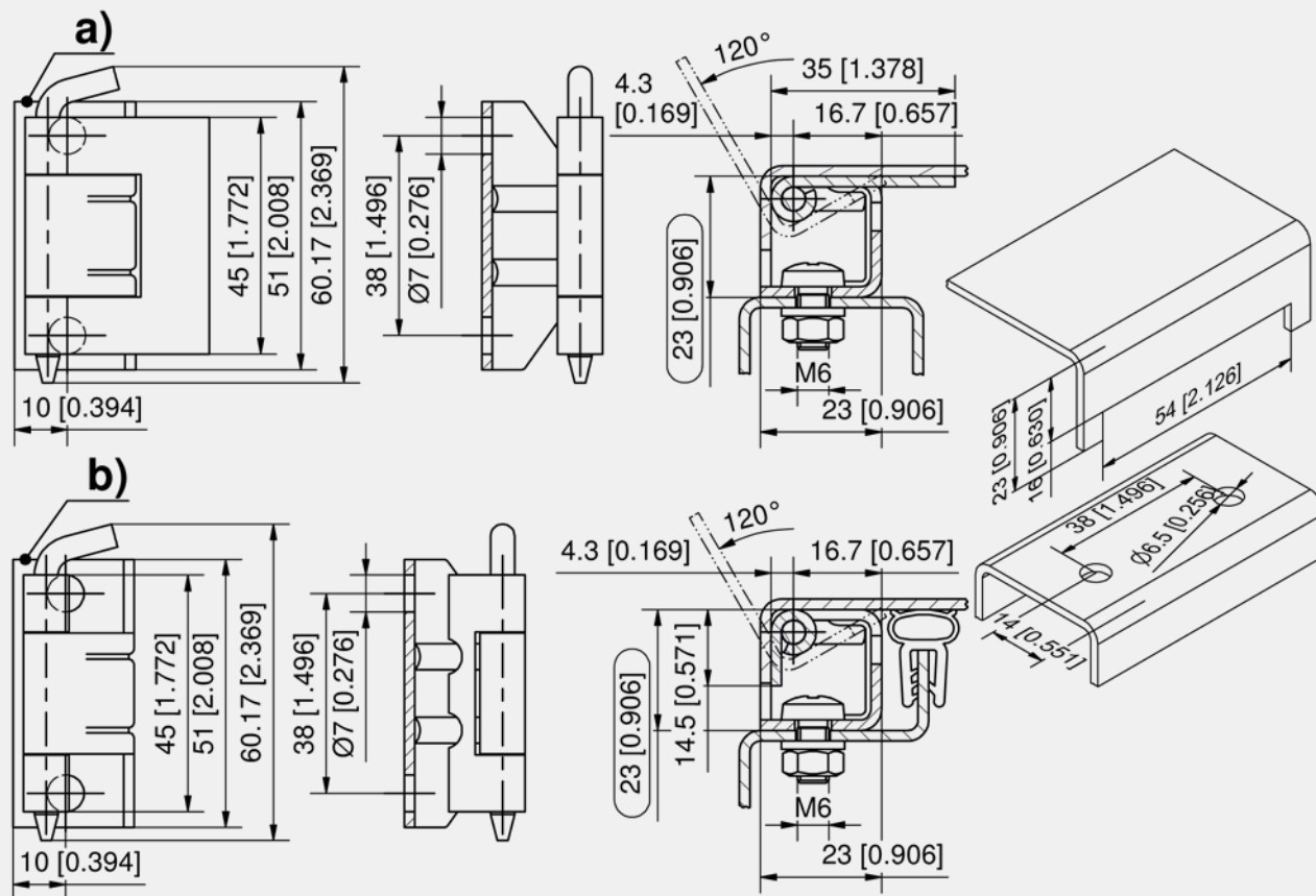
Concealed hinge
