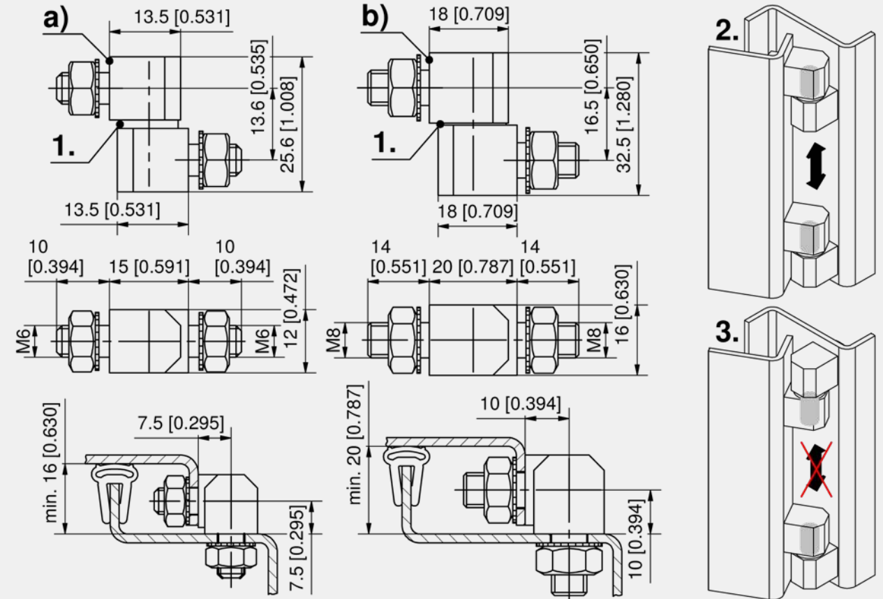
Corner hinge
