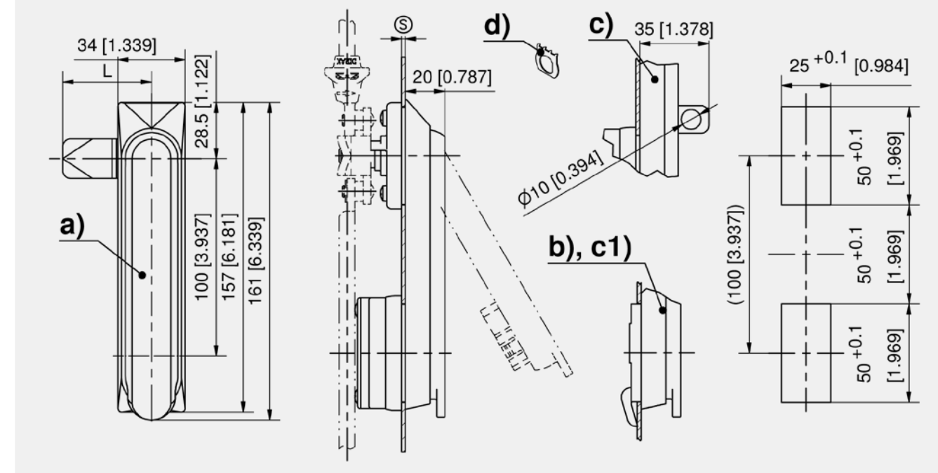
Swinghandle PA, self-locking, handle closed
