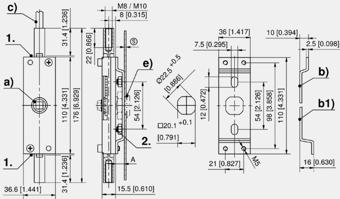
Rod latch for round rods
