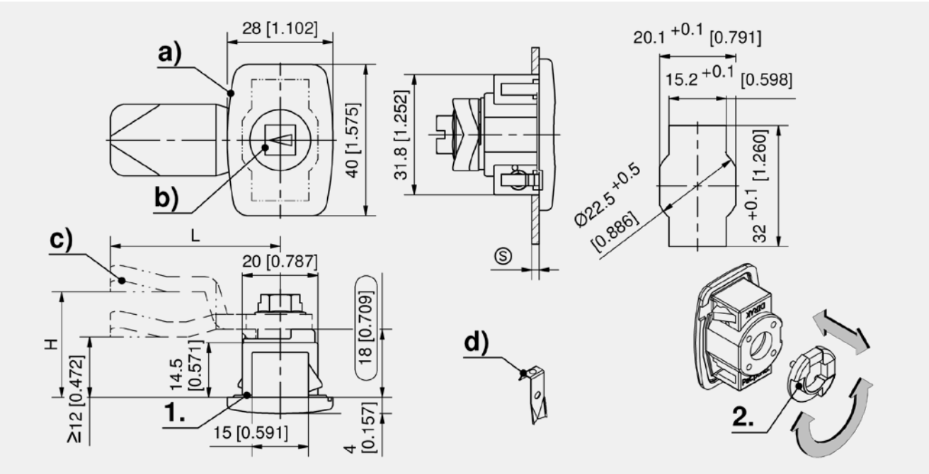
Quarter-Turn housing
