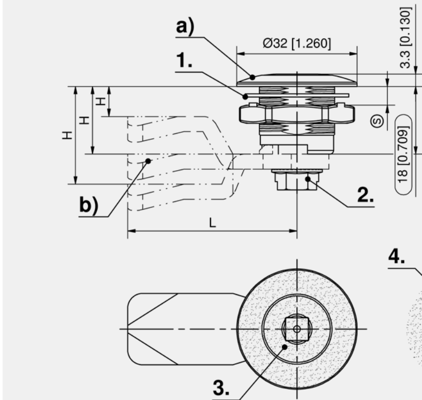
Safety quarter-turn with insert
