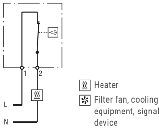
Thermostat STO 111 (NC) Connection diagram
