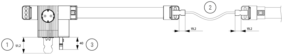
Connection example
