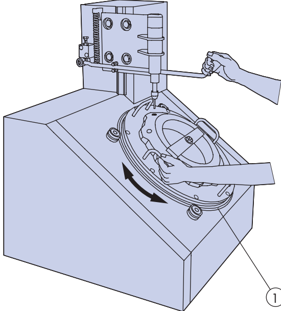
Rotary Assembly fixture HepcoMotion ring disc ① provides a large mounting area for attaching components. The precision ground surface ensures accuracy and the unhardened area inboard of the V's enables tooling holes to be drilled as required.
