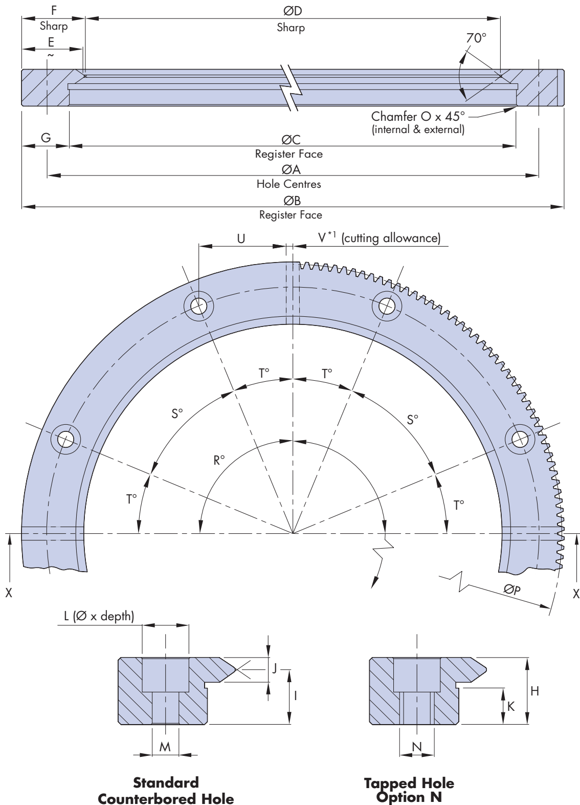
Section X-X
