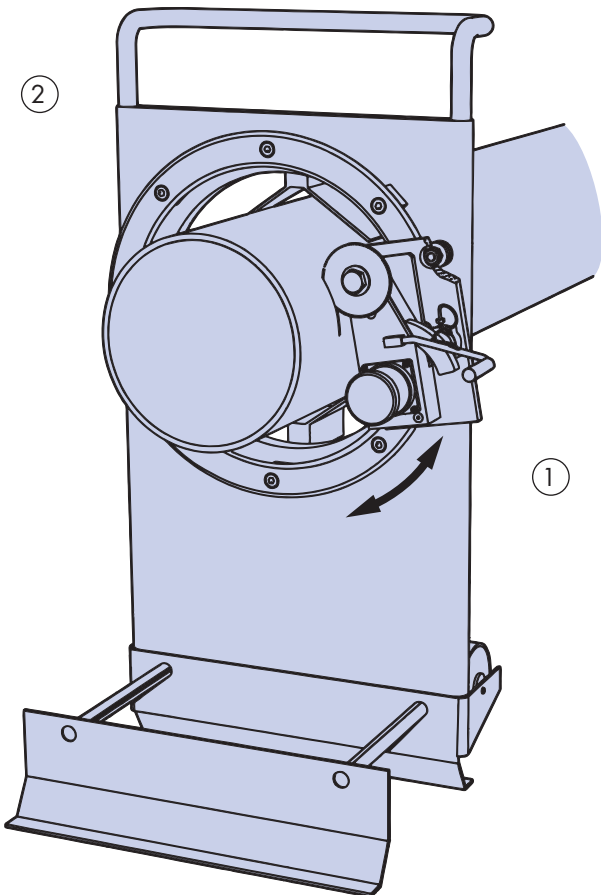
Mobile Saw for Long Tubes Motor and saw assembly mounted on carriage ① is hand operated around 360° HepcoMotion double edge ring slide ② in order to cut tube.
