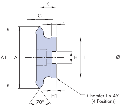
Dowel Pin 3 (SDP)
