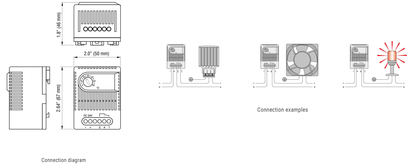
Connection diagram
