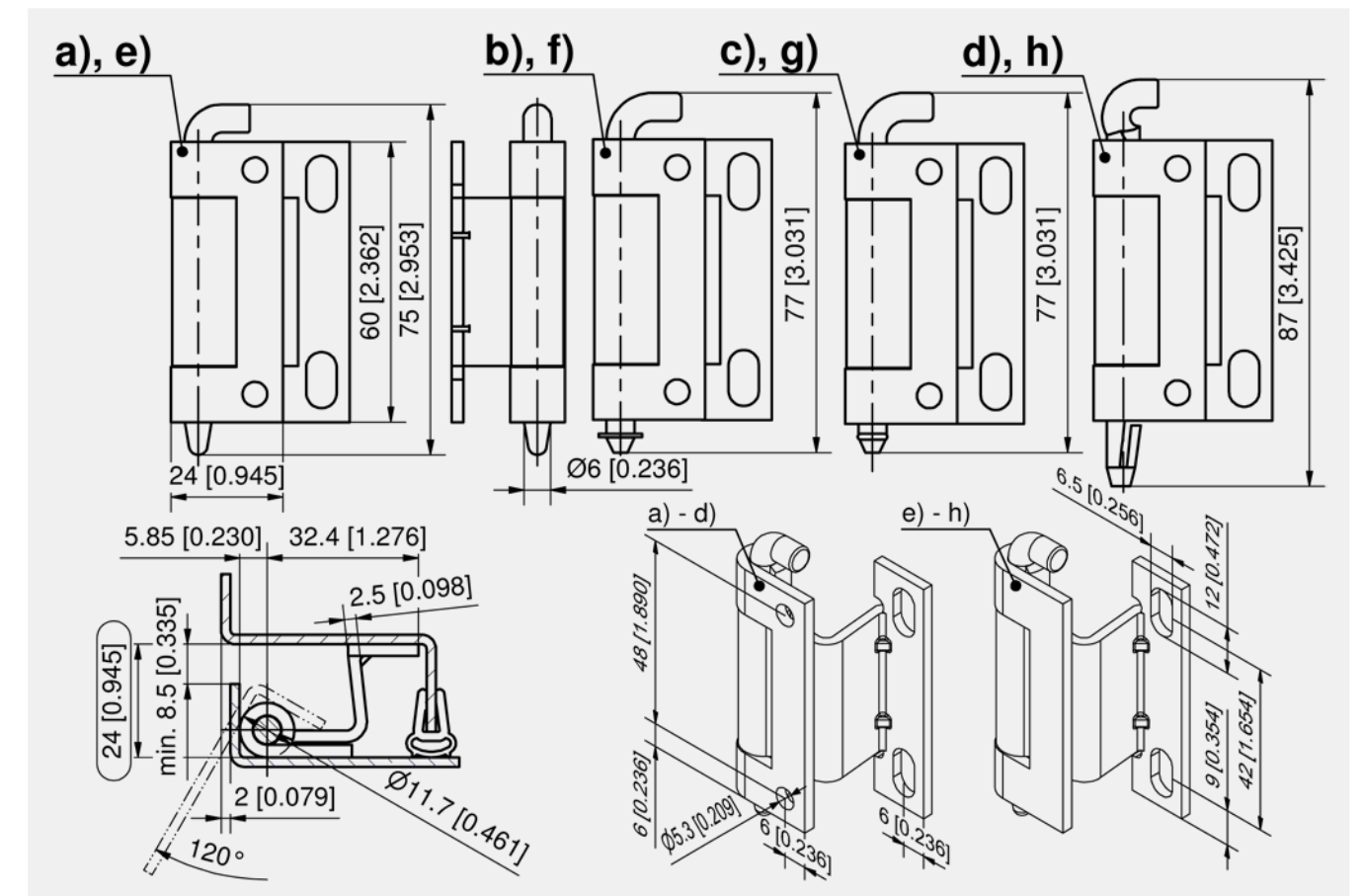
Concealed hinge
