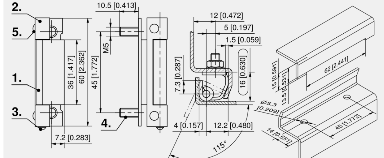
Concealed hinge
