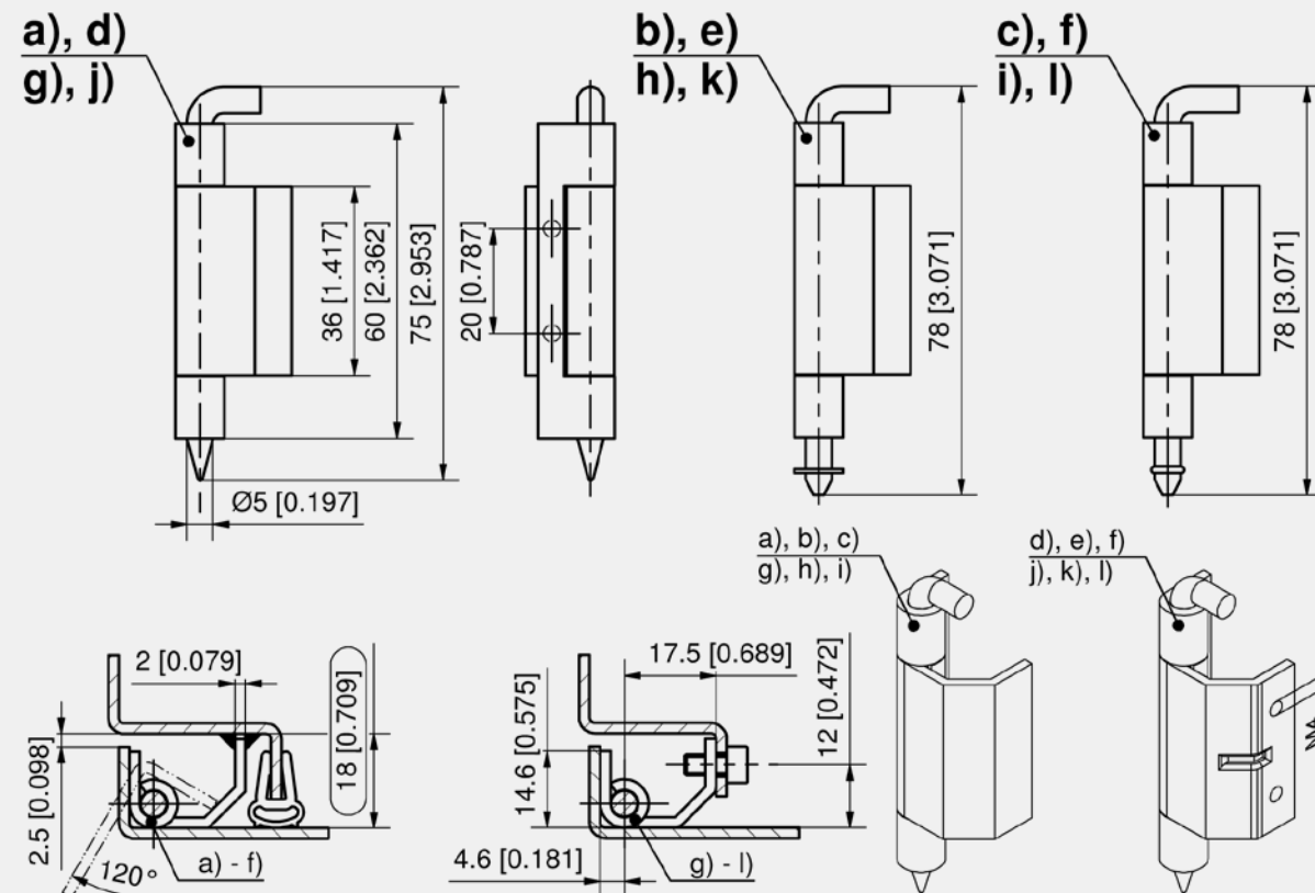
Concealed hinge
