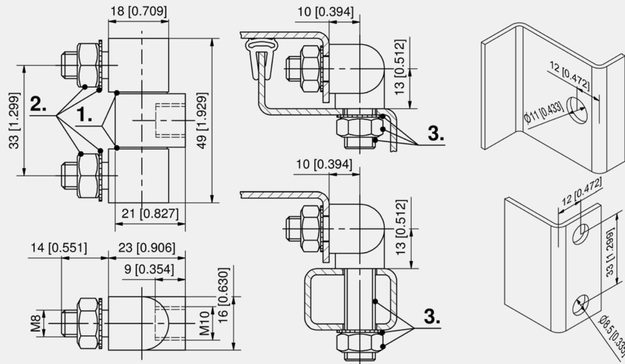
Corner hinge
