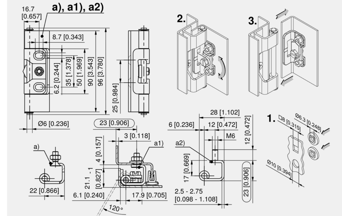
Concealed hinge
