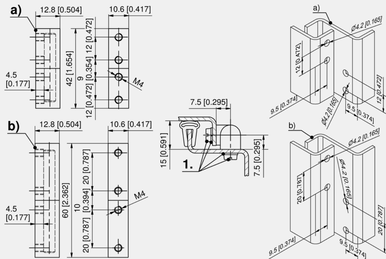
Corner hinge
