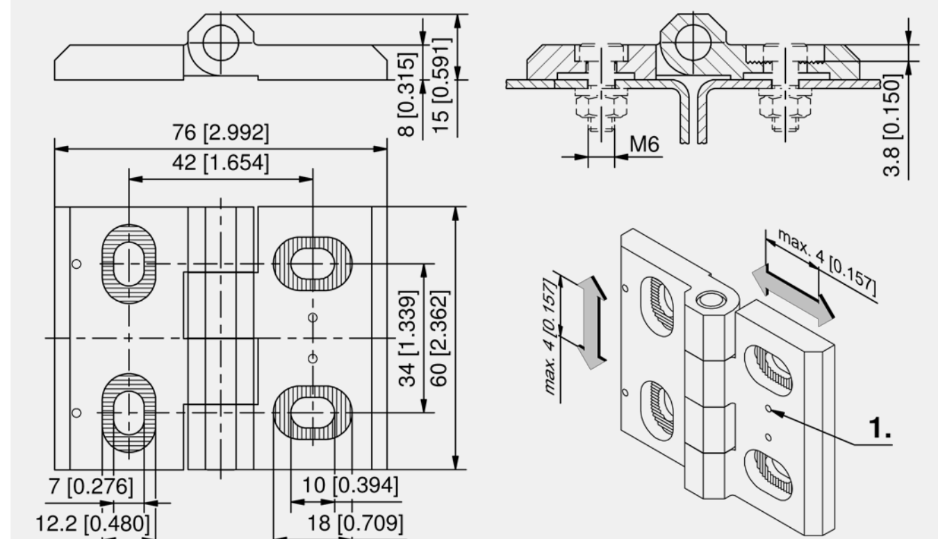
Hinge, adjustable
