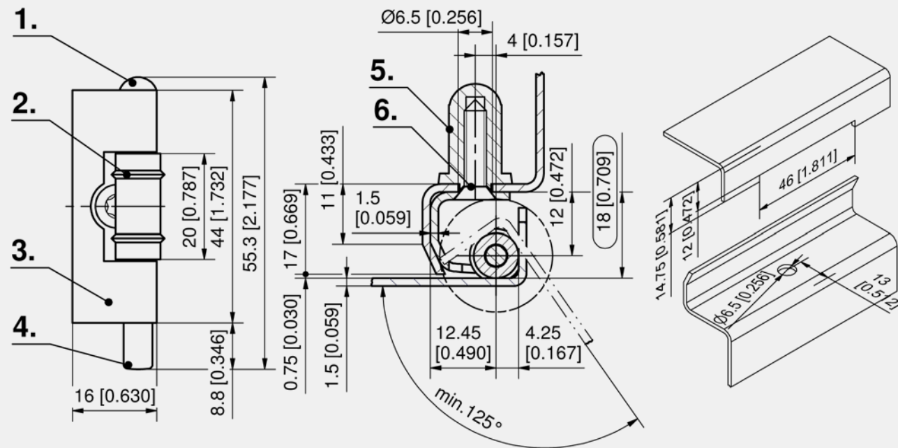
Concealed hinge
