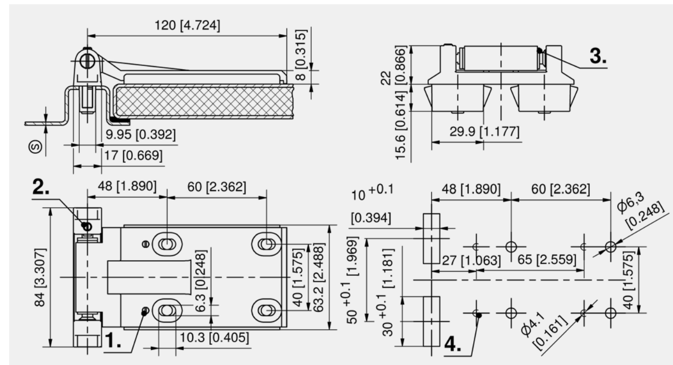
3D hinge
