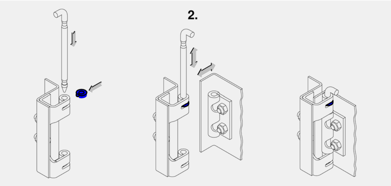
Concealed hinge
