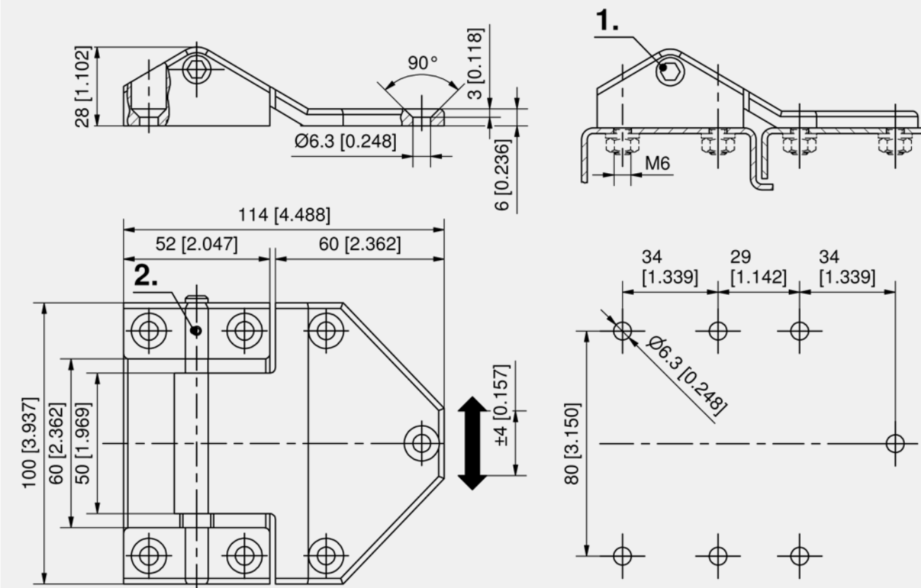
Hinge, adjustable
