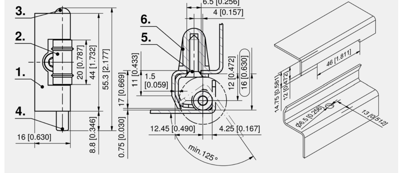
Concealed hinge
