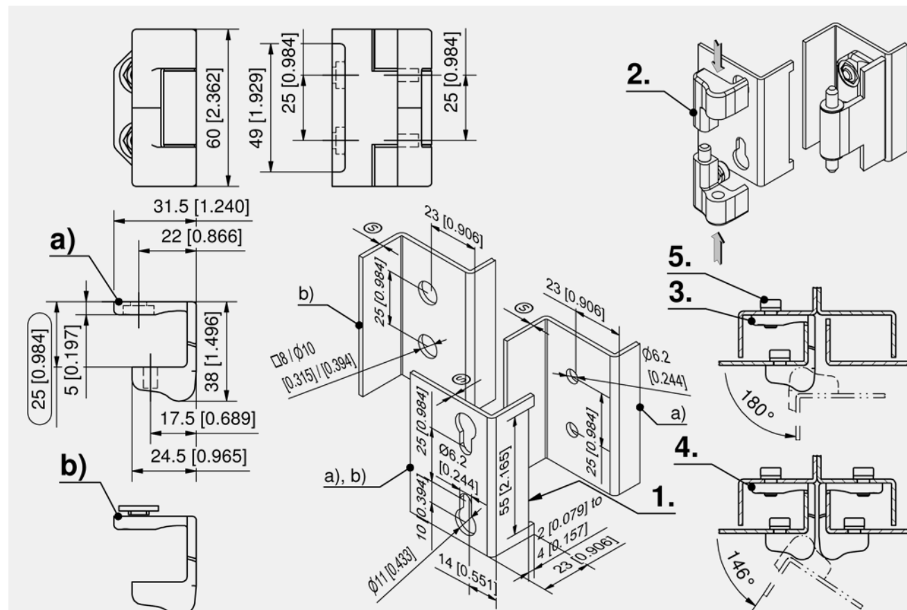
Part Number Version Pin version Installation type Delivery Unit a) 212-9302.00-00000 without fastening washer pressed in screw-on 12 pcs. b) 212-9303.00-00000 with fastening washer pressed in screw-on 12 pcs.
