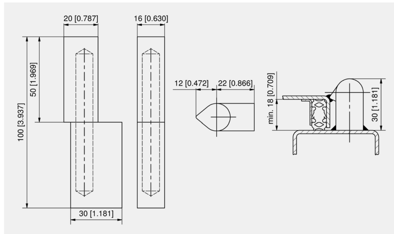
Corner hinge
