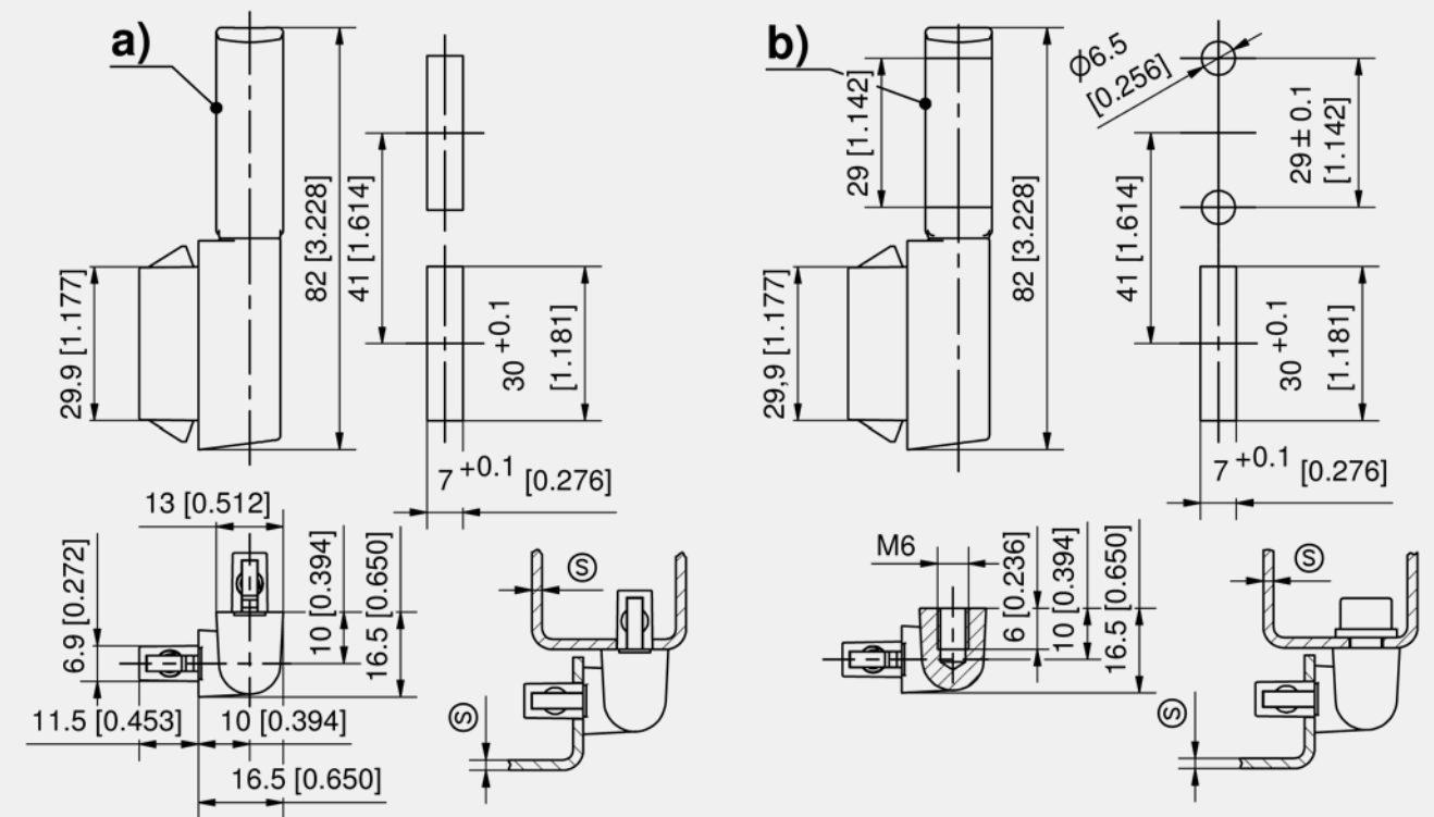
Corner hinge
