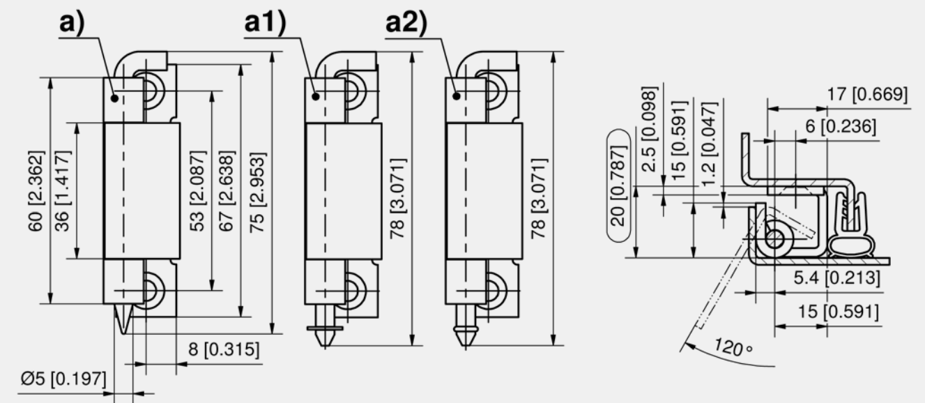
Concealed hinge
