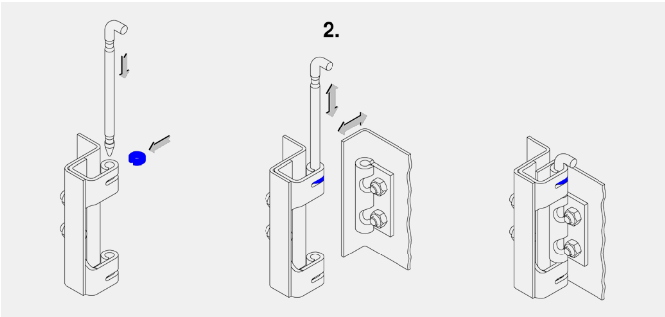
Concealed hinge
