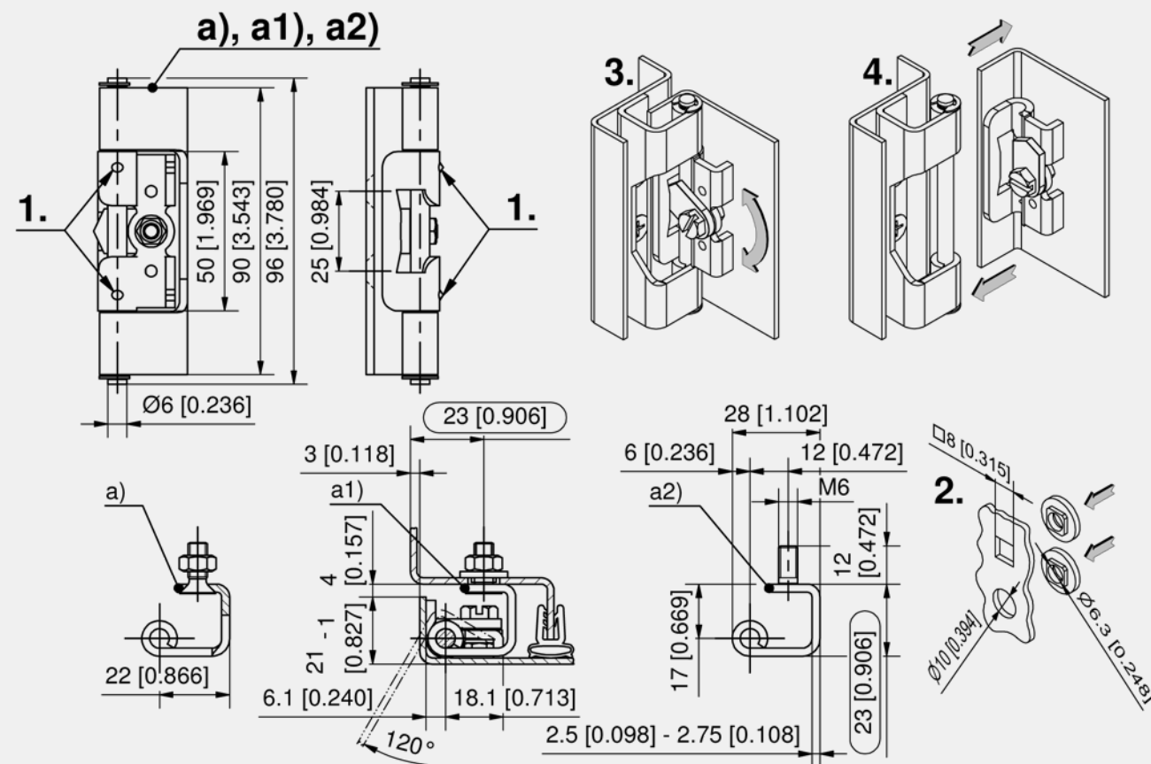
Concealed hinge
