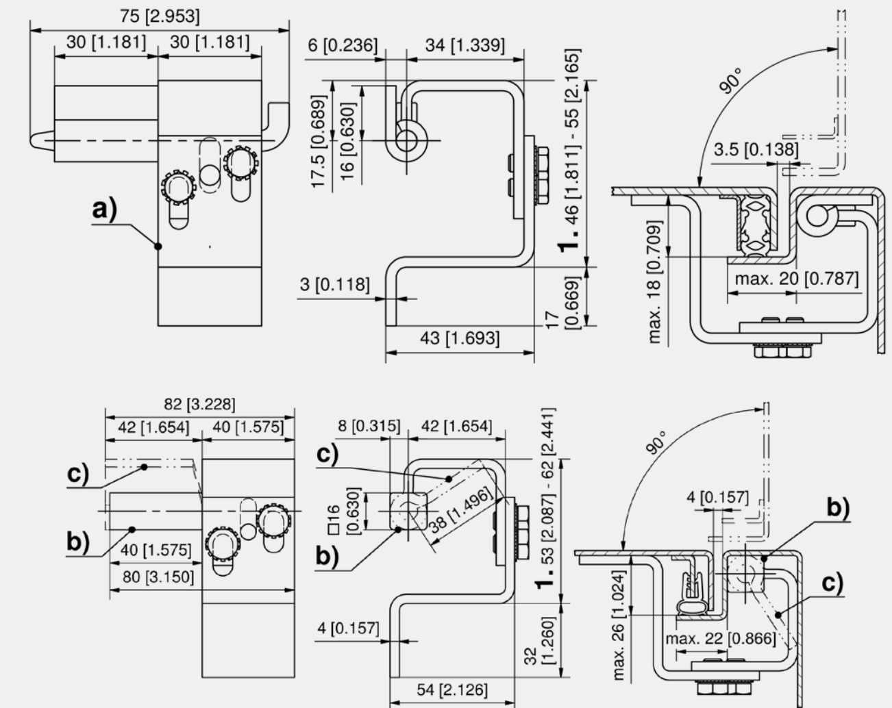
Concealed hinge
