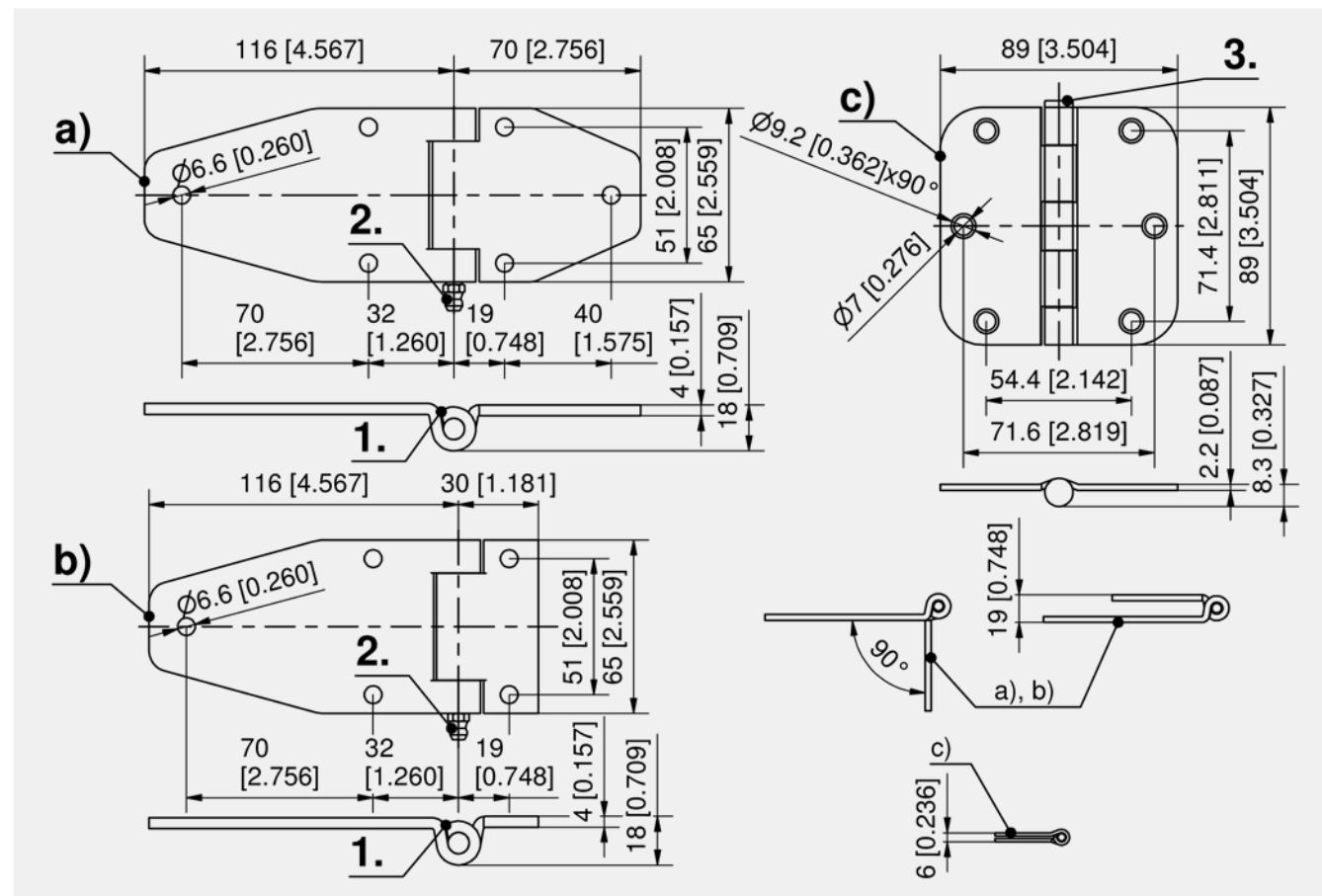
Hinge, steel
