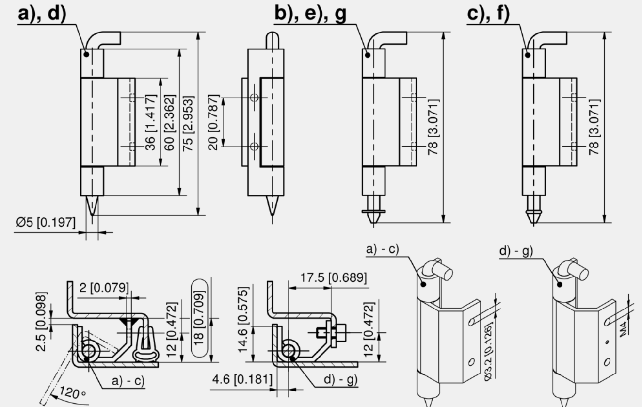
Concealed hinge
