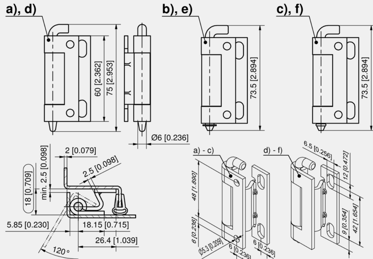
Concealed hinge
