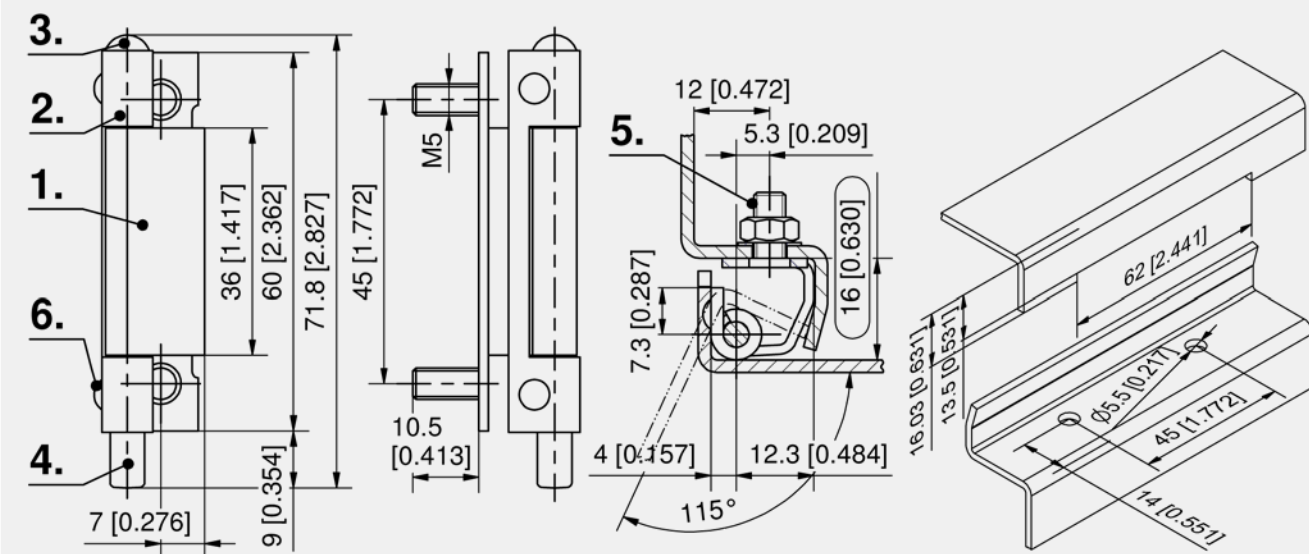
Concealed hinge
