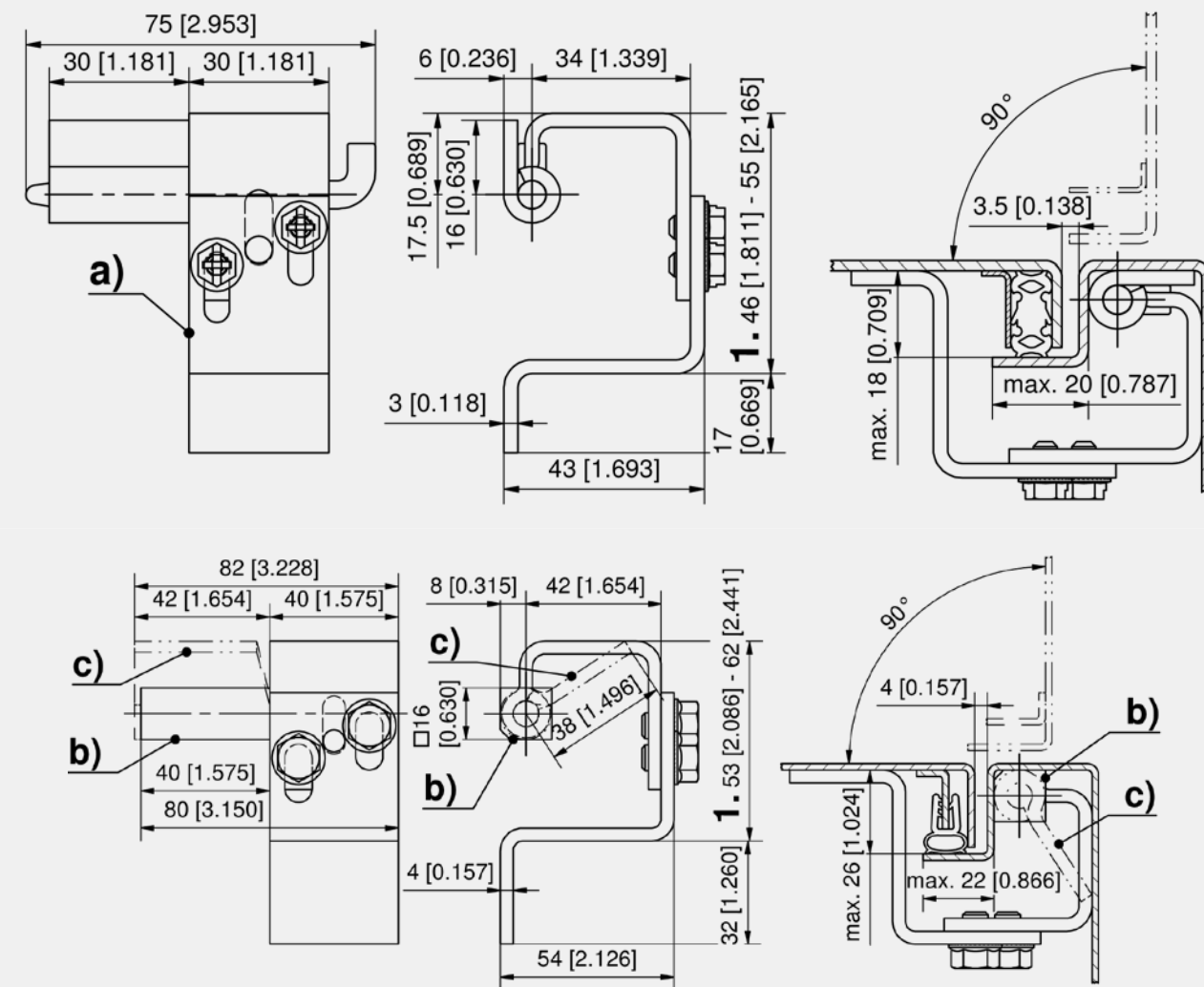
Concealed hinge
