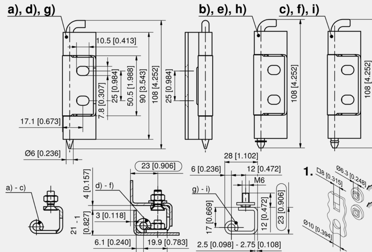
Concealed hinge
