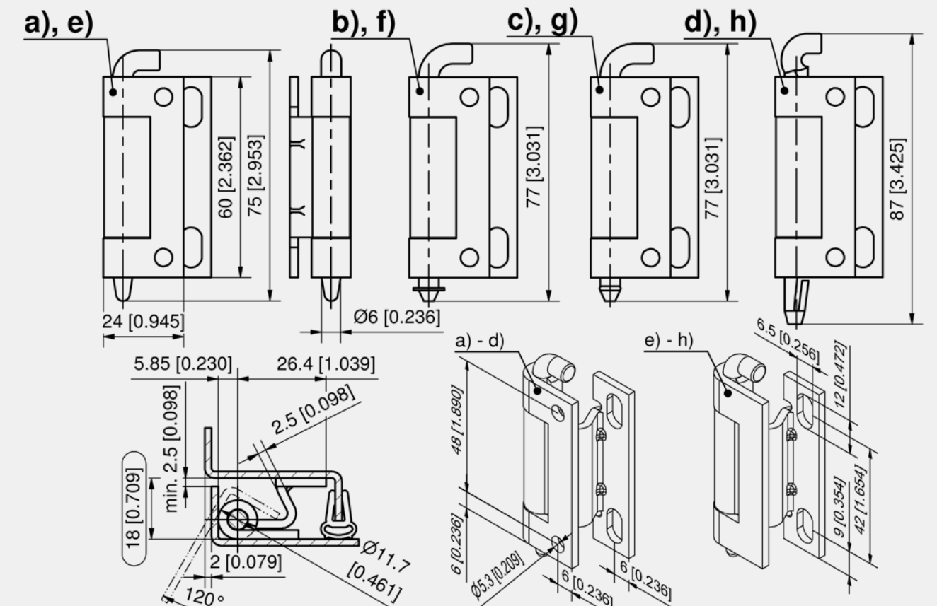
Concealed hinge
