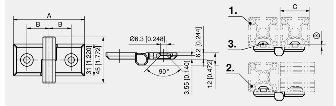
Hinge, zinc die, blasted chrome plated
