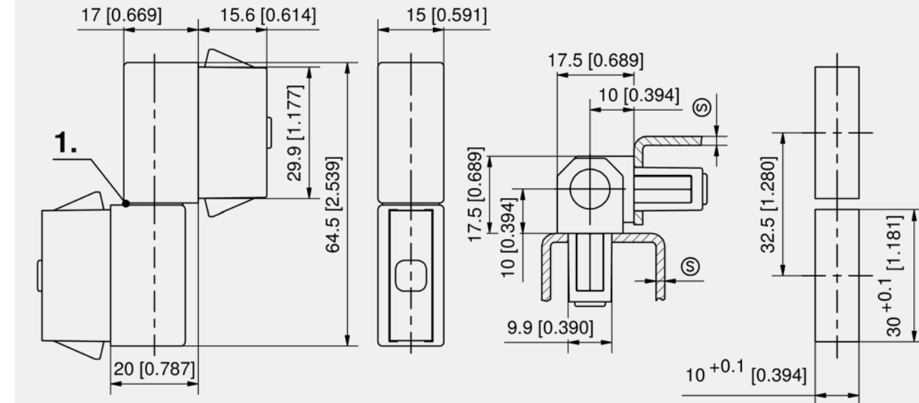
Corner hinge
