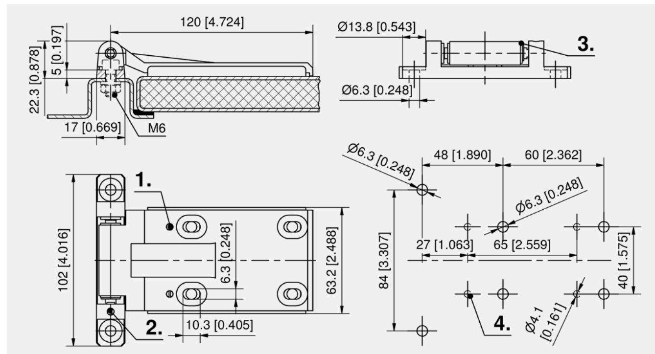
3D hinge
