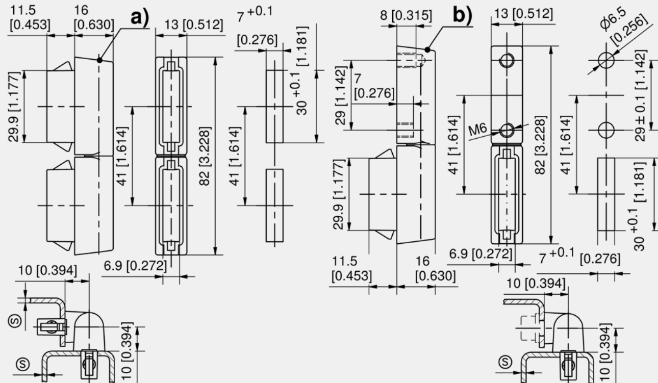
Corner hinge
