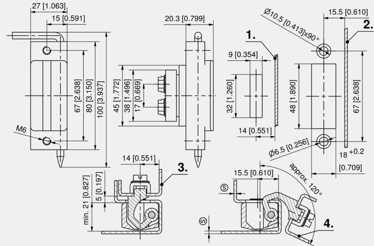
Concealed hinge
