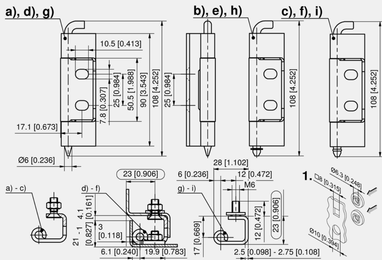
Concealed hinge
