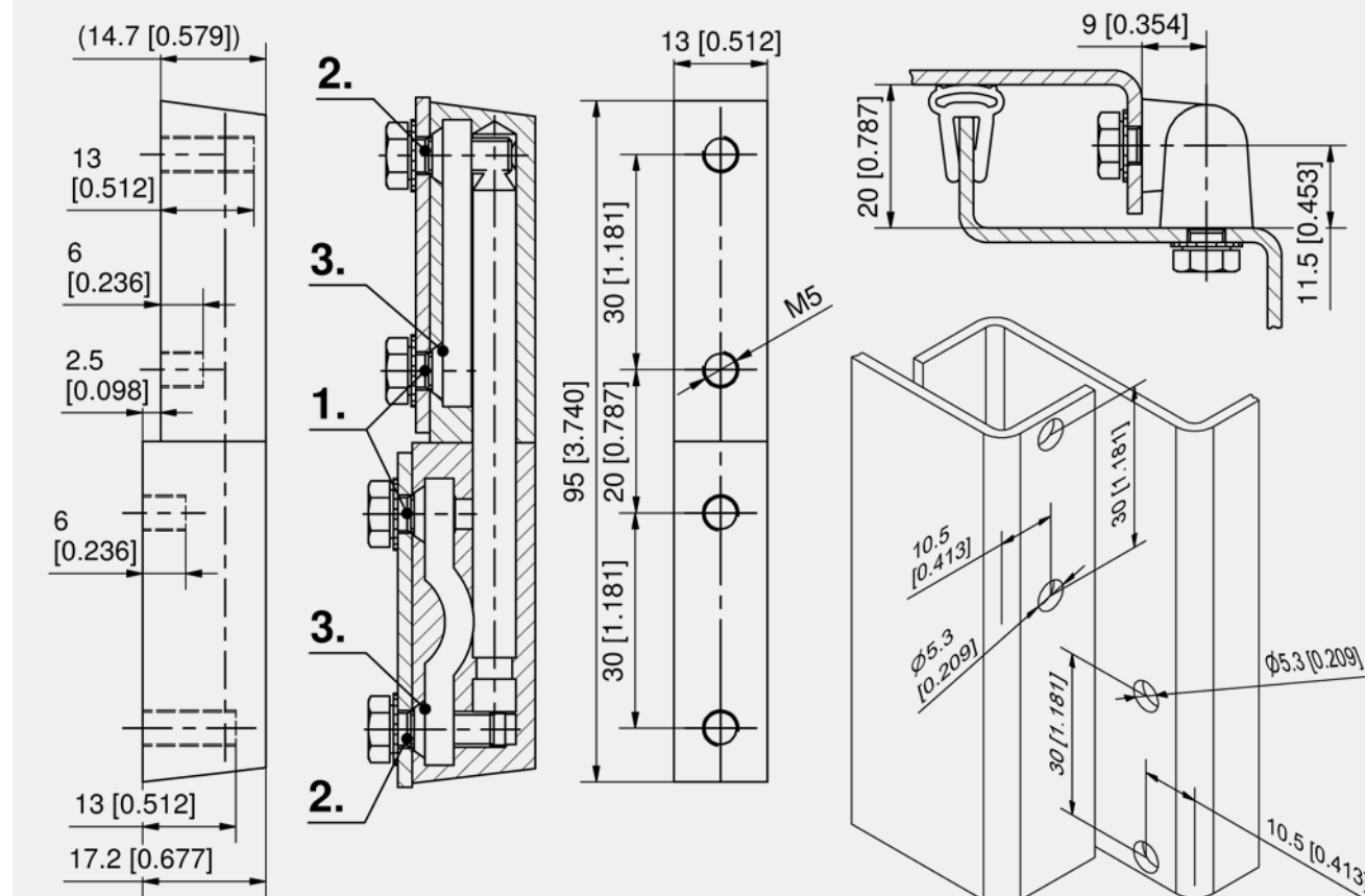
Corner hinge
